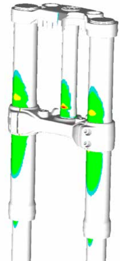
Fatigue result examples for motorcycle components obtained using FEMFAT
