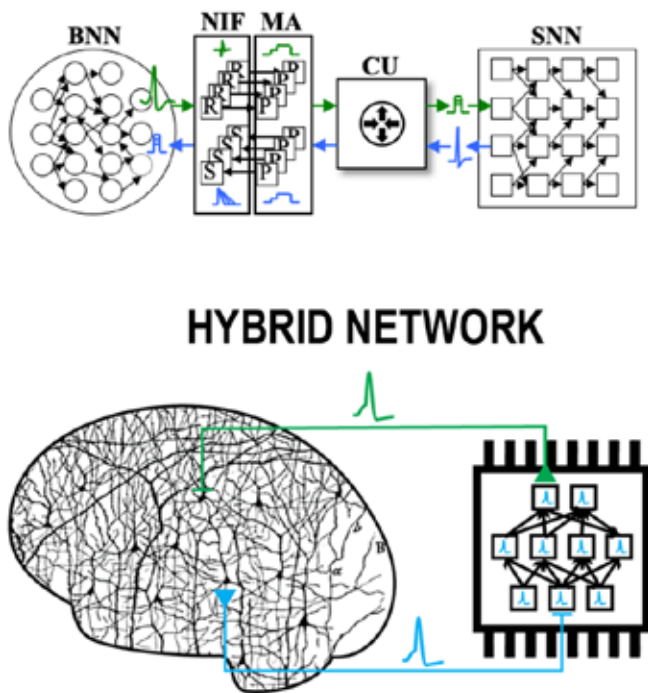
Fig. 2. SYNCH system diagram showing the NIF (neural interface); MA (memristor array platform); CU (control unit); BNN (biological neural network); and SNN (silicon neural network). In our context, the BNN is a biological network in a rat's brain (the somatosensory cortex of an anaesthetized animal at UNIPD, and the basal ganglia of a free-behaving animal at BIU), while the SNN is DynapSE hardware provided by SYNSENSE. The MA is controlled by an ARC board (SOTON and ARC).
