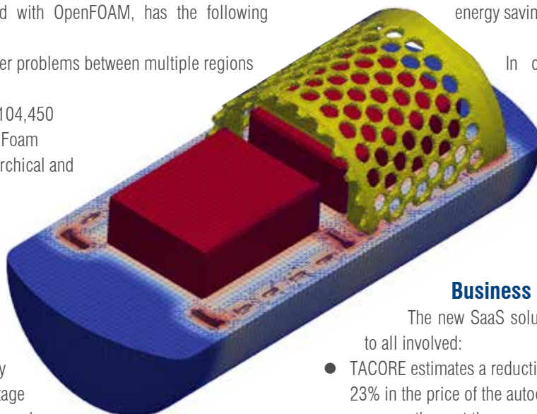
Fig. 4. Simulation mesh.
