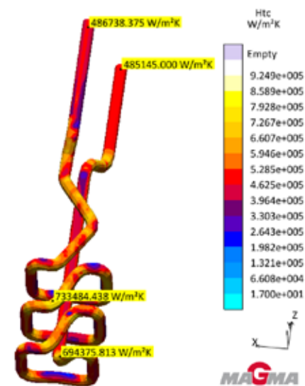
Fig. 4. Fluid dynamics study in terms of heat exchange.
