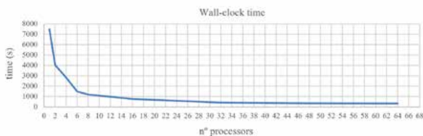
Fig. 5. Clock time vs. number of processors.
